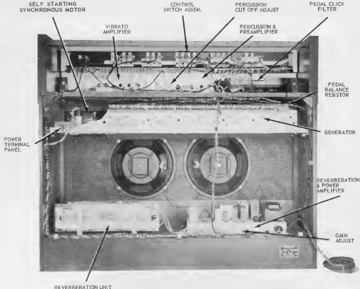
Figure 1-2. L-100 Console, Rear View
