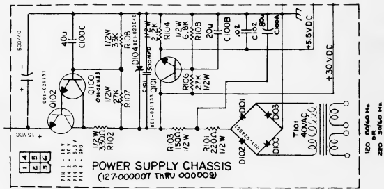
Figure 5-7. Schematic Diagram, L-100-1 Percussion Power Supply
